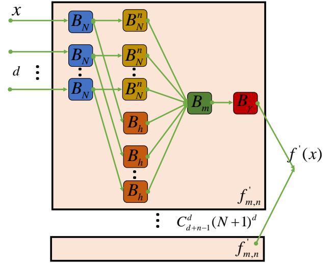
Figure 7: Strategy of using a quantized quadratic network to implement f'(\mathbf{x})
