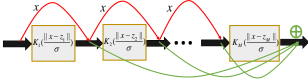
Figure 3: Quadratic ReLU network with no more than four neurons using shortcuts in each layer is universal approximator. The red shortcuts are used for passing the input and the green shortcuts for aggregating the outputs of different modules.
