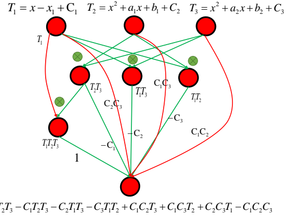
Figure 5: Quadratic network with shortcuts to learn the soft factorization of an exemplary univariate polynomial.
