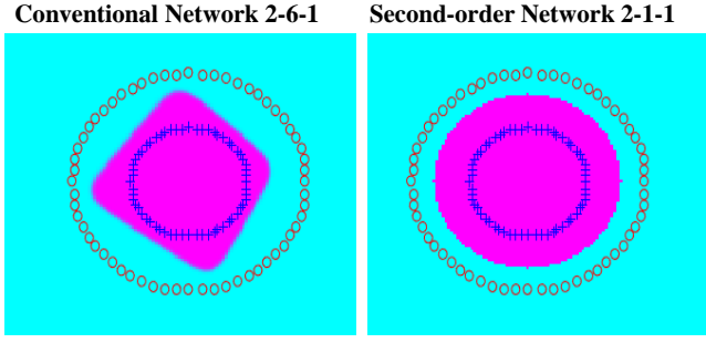
Figure 1: Classification of two concentric rings with conventional and quadratic networks ( d=2 ). To succeed in the classification, a conventional network requires at least 6 neurons (Left), and a quadratic network only takes one neuron.
