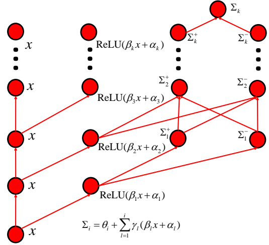
Figure 2: Illustration of a conventional network structure that allows to implement any continuous univariate piecewise linear function
