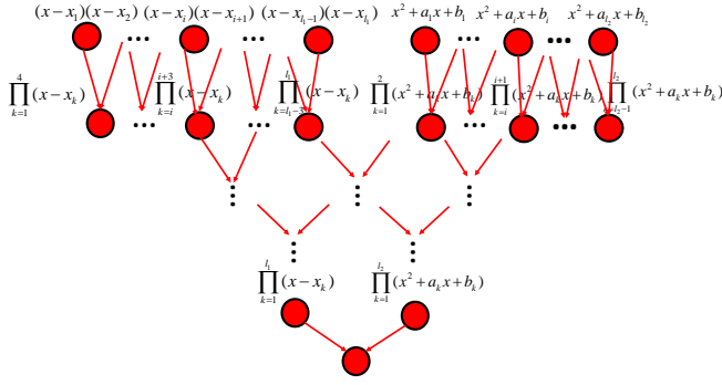
Figure 4: Quadratic network approximating a univariate polynomial according to the Algebraic Fundamental Theorem.
