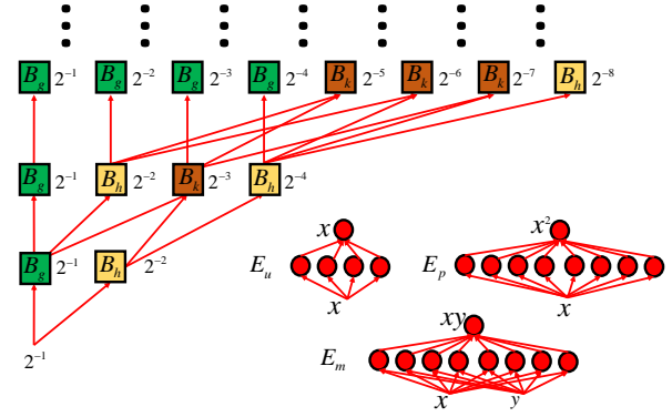
Figure 6: Quantized quadratic ReLU networks with weight 2^{-1} and -2^{-1} to approximate any number with an error bound of 2^{-t}
